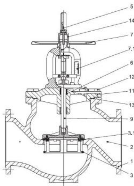
DN = 200-400 mm
