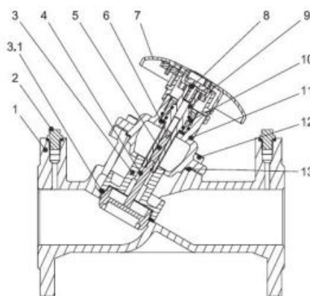
DN = 65 mm
