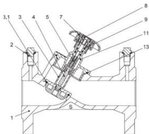
DN = 15-50 mm
