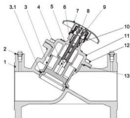
DN = 80-150 mm
