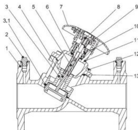
DN = 65 mm
