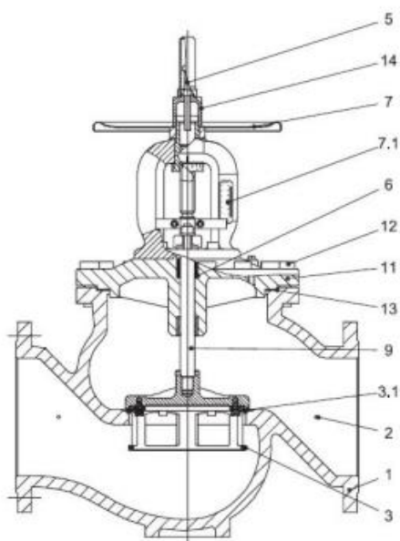
DN = 65 mm
