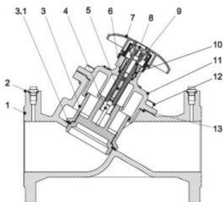
DN = 80-150 mm
